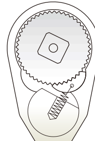
American Type Lever Change Ratchet Handle
