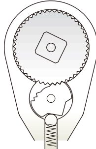
Gear to Gear Lever Change Ratchet Handle
